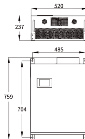
100-150A Wall-mounted
