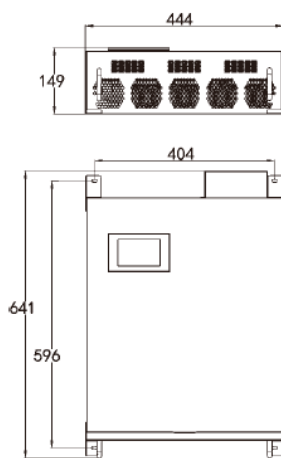
30-75A Wall-mounted
