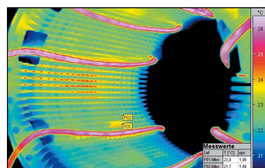
Temperature monitoring of drives
