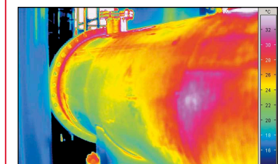
Insulation defect
