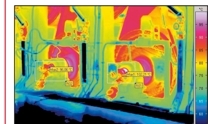
Insulation defect
